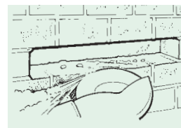
Step 1 - Three bricks are removed from the wall forming a 675mm opening (an angle grinder/cutter is ideal for cutting out).
