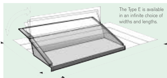
Type E cavitrays used without flashing, over an existing opening where the original damp course has failed or has been omitted. The exact course in which the cavitray is introduced varies depending on the construction detail.
