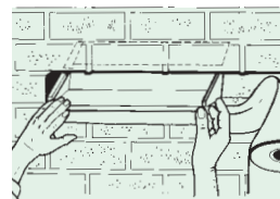
Step 2 - One cavitray is inserted together with the flashing intended for dressing over the skirting of the roof finish (flashing approx 50mm into wall). Lead flashing is not required in most remedial applications.
