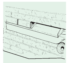
Step 3 - Two bricks are replaced in the wall into the cavitray. They are jointed and securely slate pinned, leaving the wall above safe and firm. A weepvent is incorporated in the middle perp. Two more bricks are removed again forming a three brick space. The flashing is extended and a second cavitray inserted. The integral U clip joins the trays, ensuring that no water can penetrate. Two more bricks are inserted and a weephole again formed. There are now two adjoining but completely self-contained cavitrays. The method is continued until the required run is completed. (Always bed on mortar. Do not dry bed)
